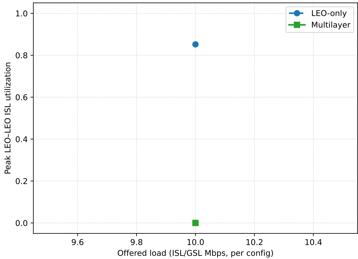
Figure L (detail) — LEO mesh peak utilization vs load — 25 s sim, 1000 ms state updates
